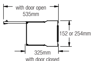
single duct dimensions
