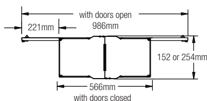
dual duct dimensions
