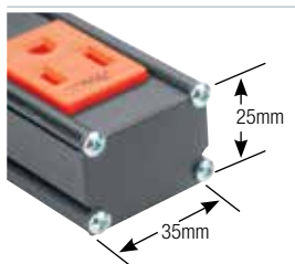
PDT 15 Amp dimensions
